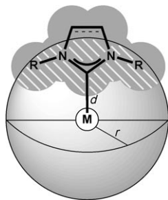
Figure 13. Graphical illustration of the buried volume (% V_{\text{bur}} ) concept.
